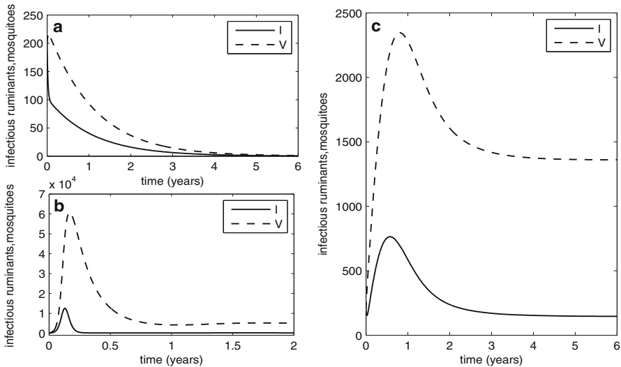
Fig. 2 Persistence of RVFV. Numerical solutions of infectious ruminants I(t) and mosquitoes V(t) : (a, b) without vertical transmission in mosquitoes ( p = 0 ) when R_0 = 0.85 ( a = 146 , p_m = 0.2 , k_0 = 0.4 ) and 17, respectively, (c) with vertical transmission in mosquitoes ( p = 0.05 ) when R_0 = 0.85 . RVFV dies out when there is no vertical transmission and R_0 < 1 and it is endemic when there is no vertical transmission and R_0 > 1 . Although R_0 < 1 , RVFV is endemic when there is vertical transmission
